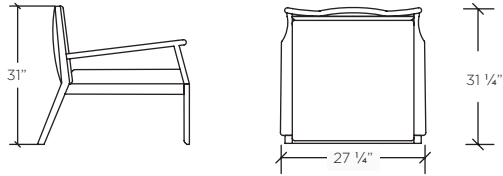
SIDE ELEVATION SEAT HEIGHT: 17"
